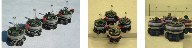
Figure 1.5. Left: four real s-bots forming a linear swarm-bot . Centre and Right: four s-bots coordinately move and avoid falling. Notice that one s-bot is suspended out of the border of the arena, and the physical connections among s-bots provide support.
