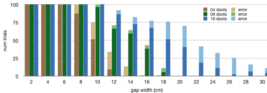
Figure 1.7. Performance of a swarm-bot passing over a trough. The stacked boxes represent the number of trials in which the swarm-bot manages to pass over the trough, and the number of trials in which an error occurs (i.e., the swarm-bot falls or remains stuck over the trough).
