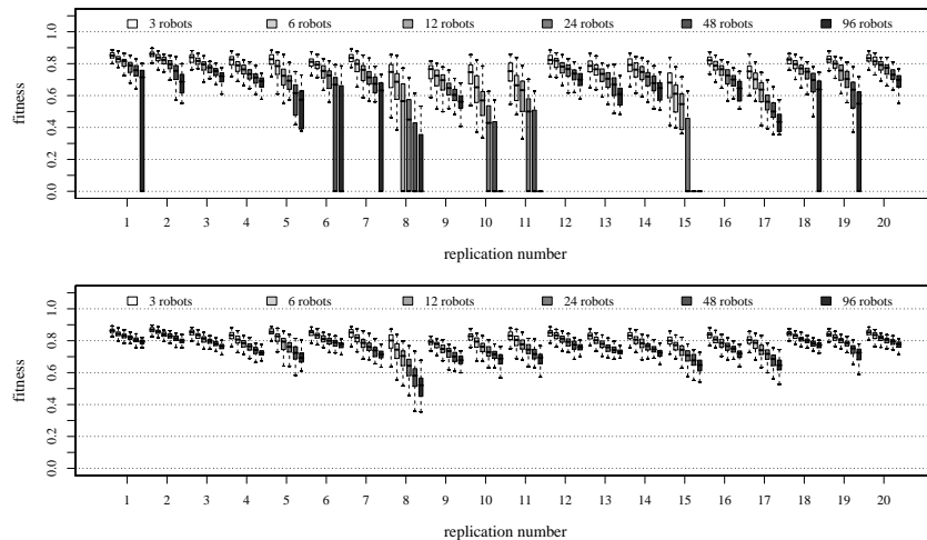
Figure 1.4. Scalability analysis for the continuous communication system. Top: scalability of the evolved controllers under normal conditions. Bottom: scalability of the synchronisation mechanism.
