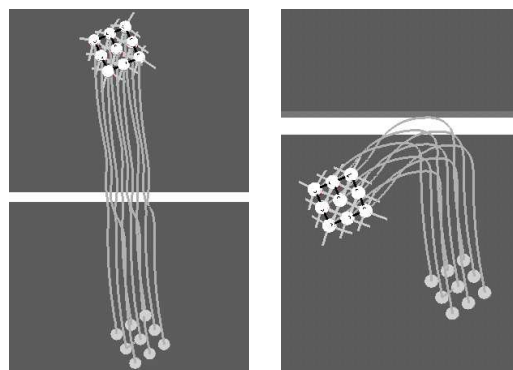
Figure 1.6. Trajectories drawn by a swarm-bot composed of 9 s-bots in a square formation. Left: the swarm-bot is able to pass over a 10 cm wide trough. Right: the swarm-bot avoids a 20 cm wide trough, which could be too large to be bridged.
