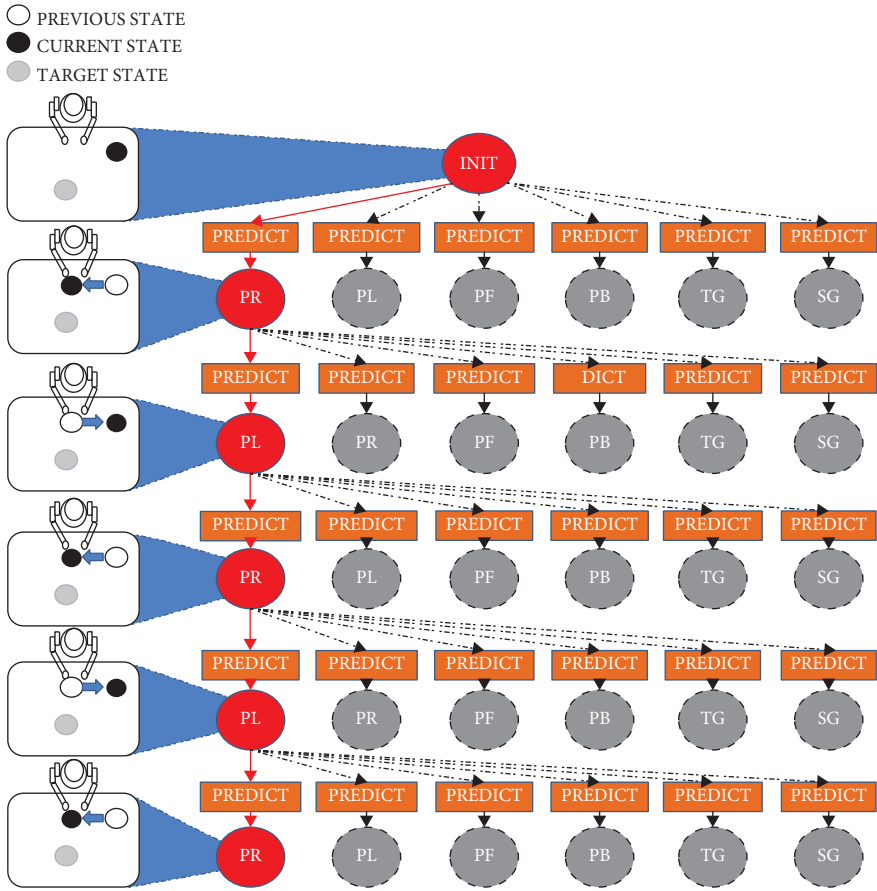
Figure 13. Multi-Step planning demonstration with naive prototype based verb concepts – C_{NP} (and the pure cMahalanobis distance in Equation 9). The behaviors are abbreviated as PR ( push-right ), PL ( push-left ), PF ( push-forward ), PB ( pull ), TG ( top-grasp ) and SG ( side-grasp ). The initial and the target states for the objects are the same with the one provided in Figure 11. Since the distance calculations yield wrong results due to irrelevant changes between the initial and goal states, the search does not terminate with success
