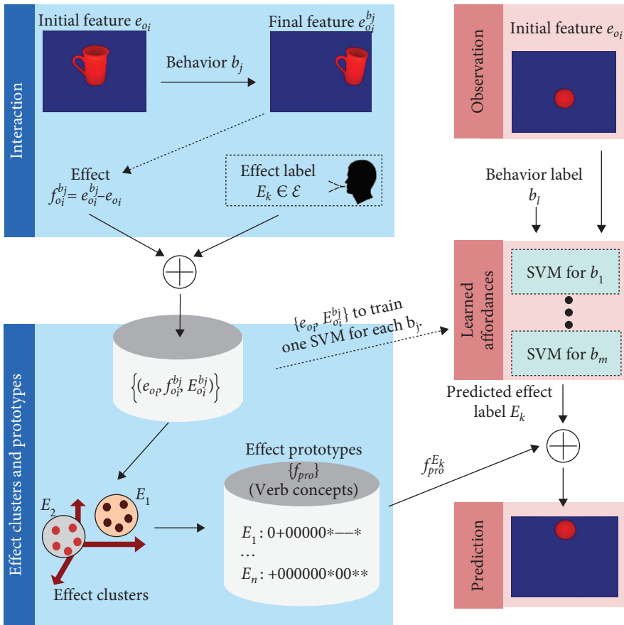
Figure 7. Clusters in the effect space are used for training an SVM, which allows the effect label to be predicted from a behavior on a novel object
