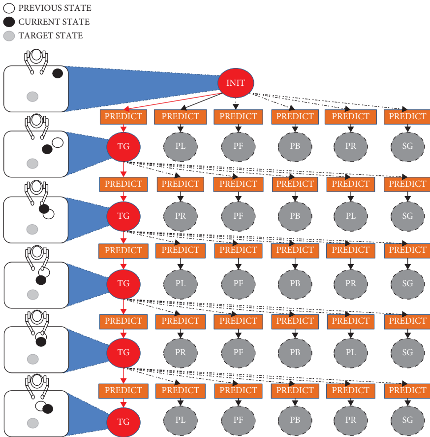
Figure 14. Multi-Step planning demonstration with exemplar-based verb concepts – C_{Ex} (and Euclidean distance in Equation 10). The behaviors are abbreviated as PR ( push-right ), PL ( push-left ), PF ( push-forward ), PB ( pull ), TG ( top-grasp ) and SG ( side-grasp ). The initial and the target states for the objects are the same with the one provided in Figure 11. Since the distance calculations yield wrong results due to irrelevant changes between the initial and goal states, the search does not terminate with success.
