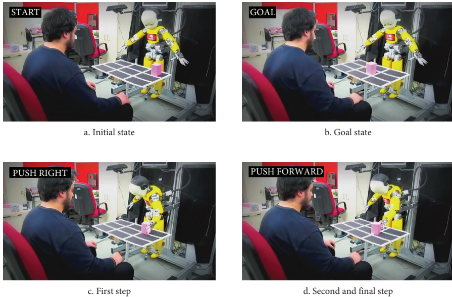
Figure 11. A sample execution of multi step planning using C_{EP} - i.e. effect prototype based verb concepts. First, the initial state (a) and final state are shown (b). Then, the robot makes a plan involving push-right and push-forward behaviors, which are executed as shown in (c) and (d). When a simple Euclidian distance or naive prototype is used, the robot could not derive a plan
