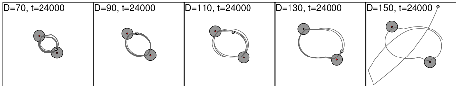
Fig. 9 From left to right, each snapshot displays the trajectory followed by a single robot in five different trials, in which the target areas are positioned according to the distance values in D_{set} . Notice the failure of the individual strategy when D = 150 cm (last frame on the right). See also the video ‘single-robot-D150.mpeg’ ( N = 1 , D = 150 cm) in the online supplementary material. For further video footage about the single robot experiment, refer to http://laral.istc.cnr.it/esm/sperati-et-al-2010
