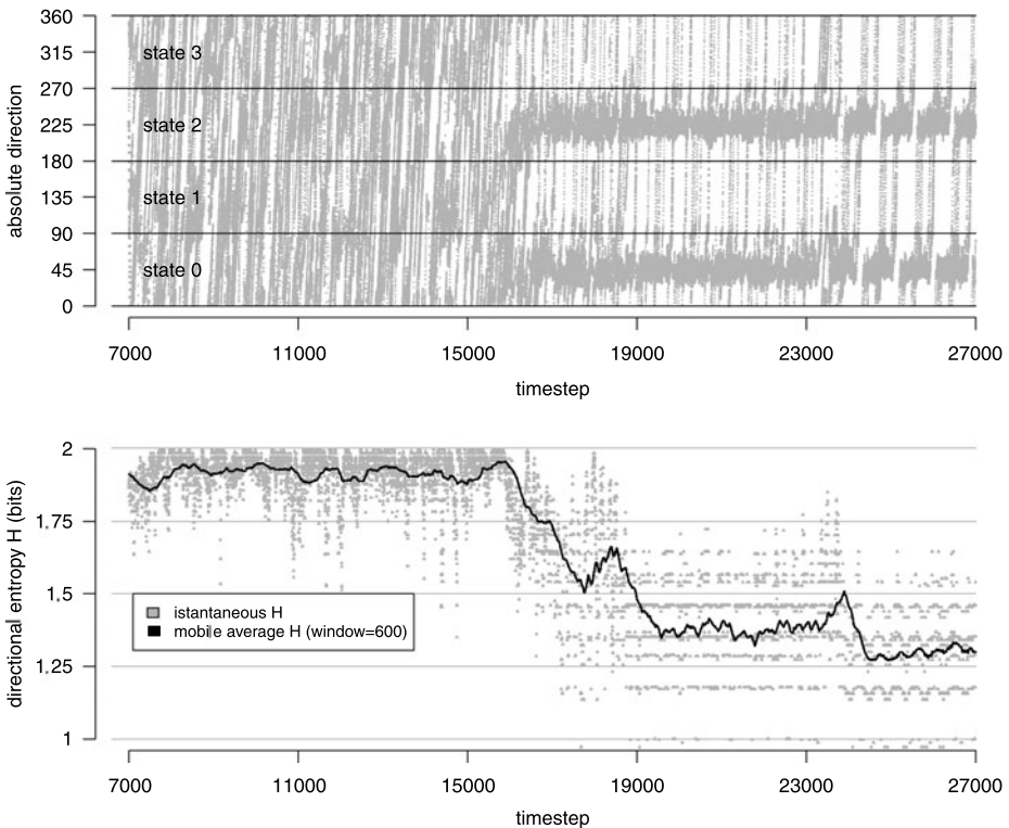
Fig. 11 Top: the absolute directions followed by robots is plotted through time (grey lines) during a successful trial ( N = 30, D = 250 ). It is possible to notice how all robots converge and maintain a heading similar to the direction between target areas once the dynamic chain is formed. The figure also shows how the heading direction is discretised in four states for the computation of the entropy H[X] . Bottom: the respective values of H[X] for each time step are drawn in grey, the moving average with a window of 600 time steps is drawn in black. The time step when the average drops to values lower than 1.75 corresponds to the formation of the chain
